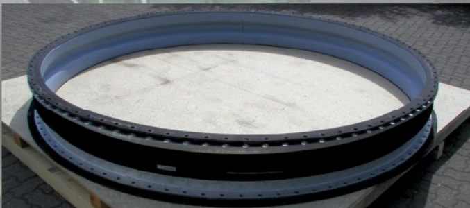
Expansion joint with vulcanised PTFE lining for chemical applications
